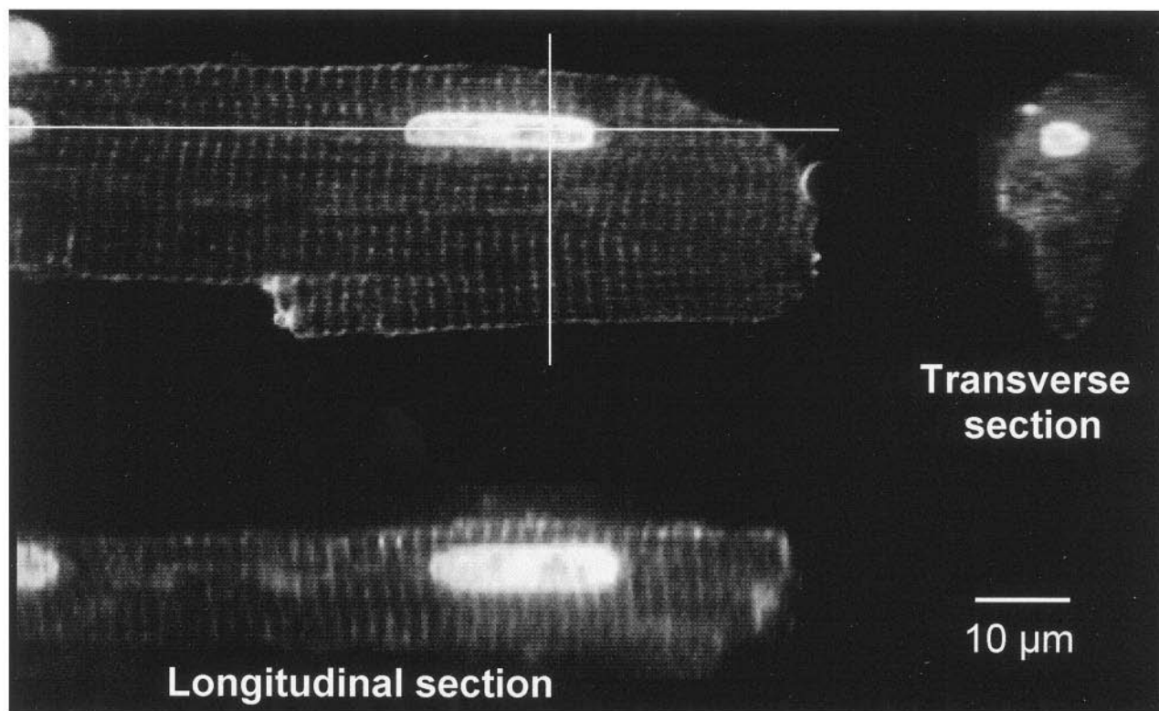
FIGURE 2 Optical slice images and reconstructions from these slice images. A rat cardiac myocyte labeled with di-8-ANEPPS (t-tubules) and SYTO 11 (nucleus) was sliced at 1 \mu\text{m} thickness intervals by Nipkow disk confocal microscopy. A shows 6 of 16 sliced images. The reconstructions of 16 images into longitudinal and transverse cross-sections were produced by computer and are shown in B .
